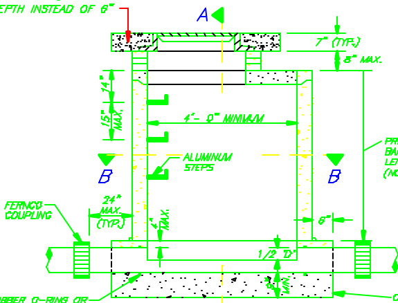
SECTION ELEVATION
